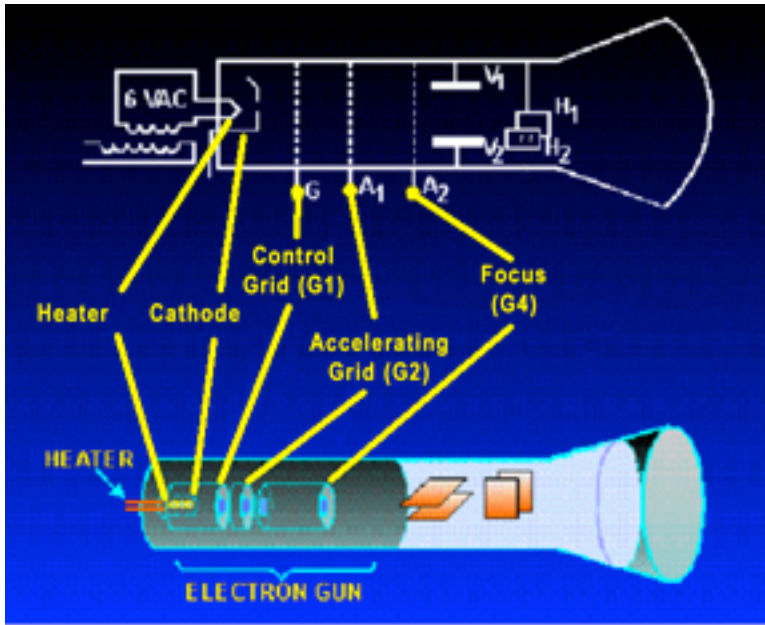
Figure 2. A CRT gun has five basic elements.
