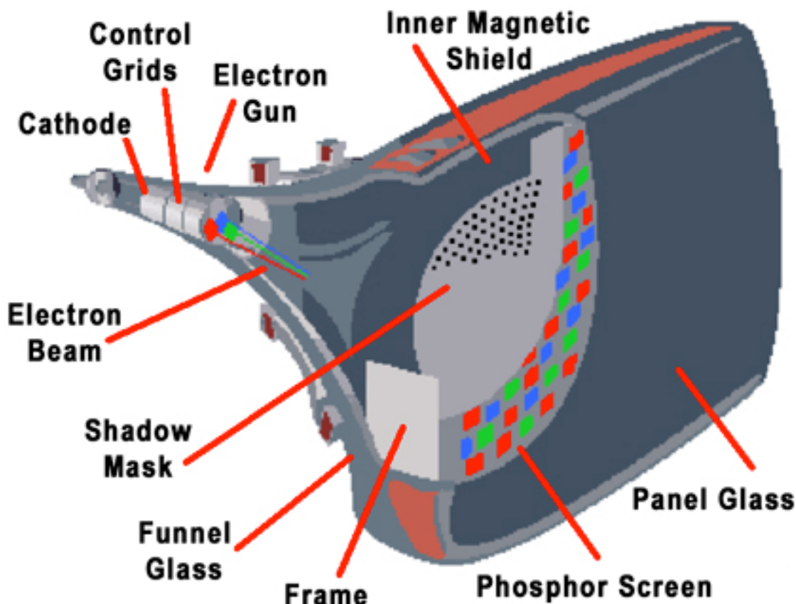
Figure 1. The electrons produced by the cathode are regulated and accelerated until they collide with the phosphor to produce light.
