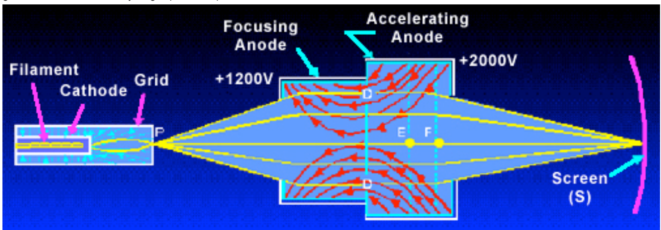
Figure 3. Electrons are attracted to the focusing anode, and travel through the small hole in the grid.
